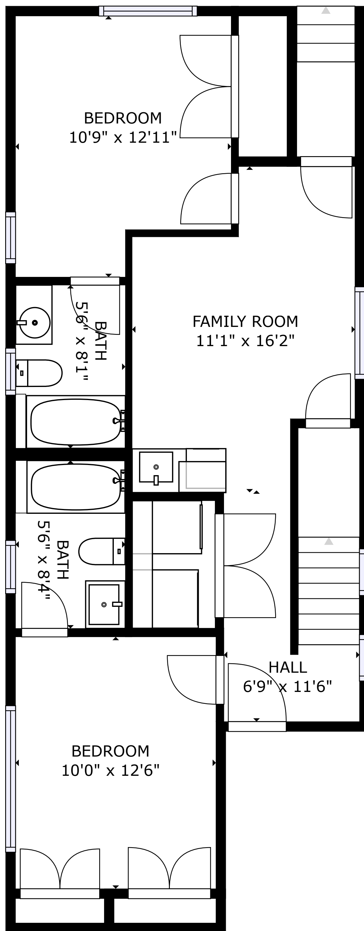
FLOOR 1
